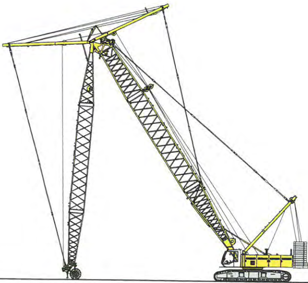
Erecting of main boom and luffing jib
